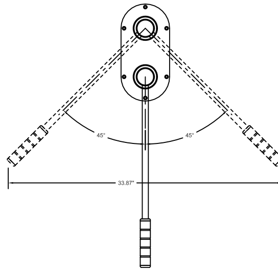
TOP VIEW SHOWN IN 1:2 SCALE
