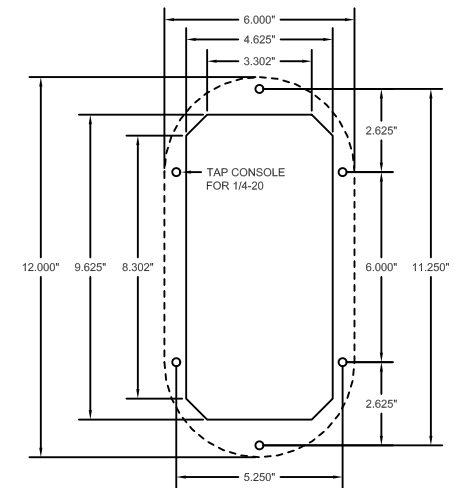
PANEL CUTOUT
