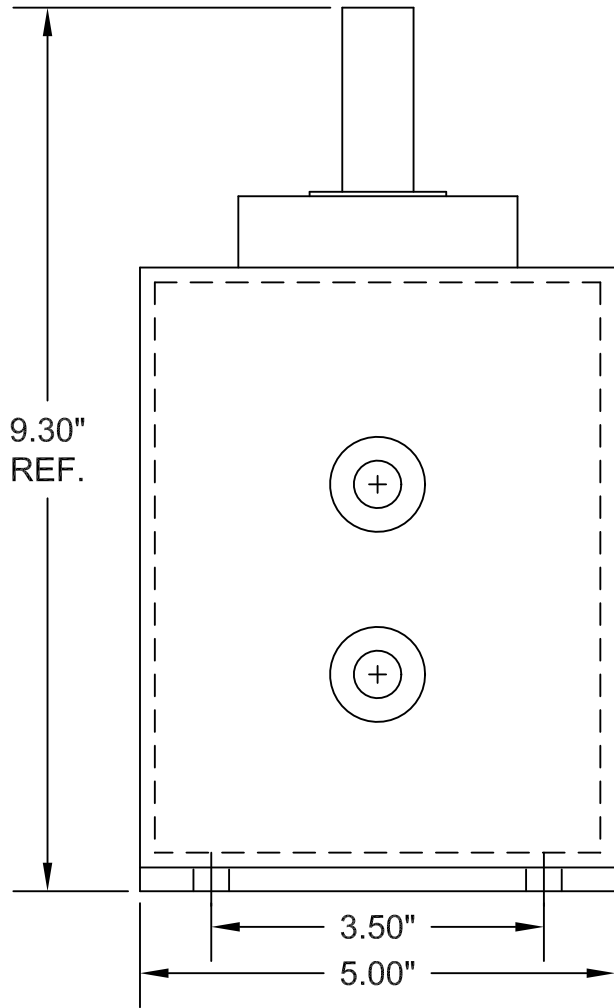
END VIEW
