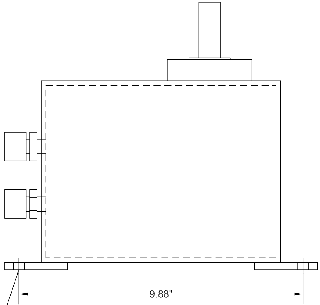
FRONT VIEW
