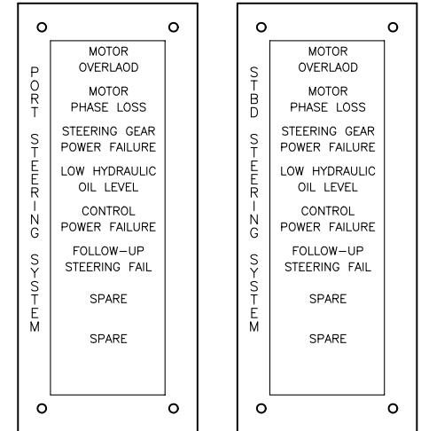
TYPICAL STEERING ALARMS (SEE NOTE 1)
