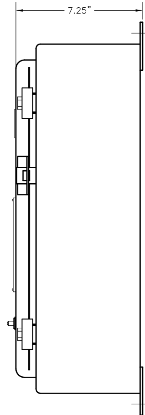
SIDE VIEW
