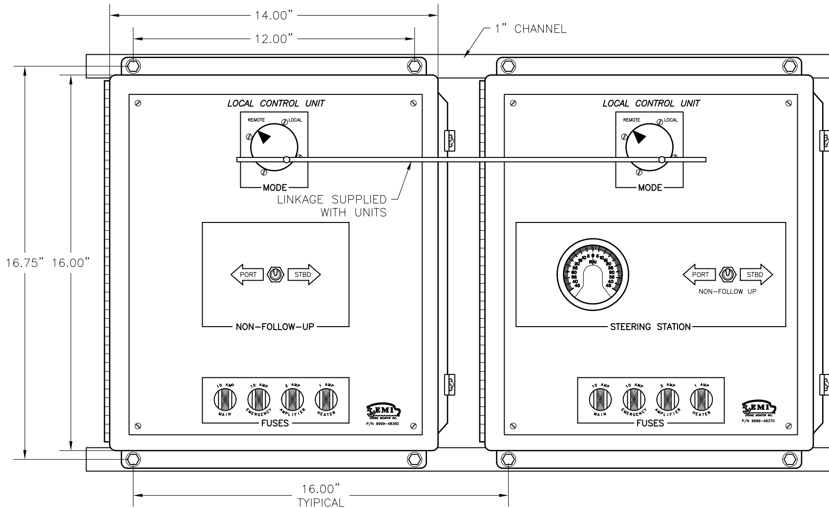
FRONT VIEW
