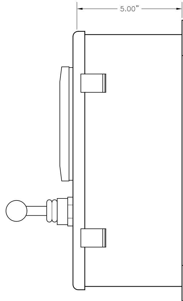
SIDE VIEW
