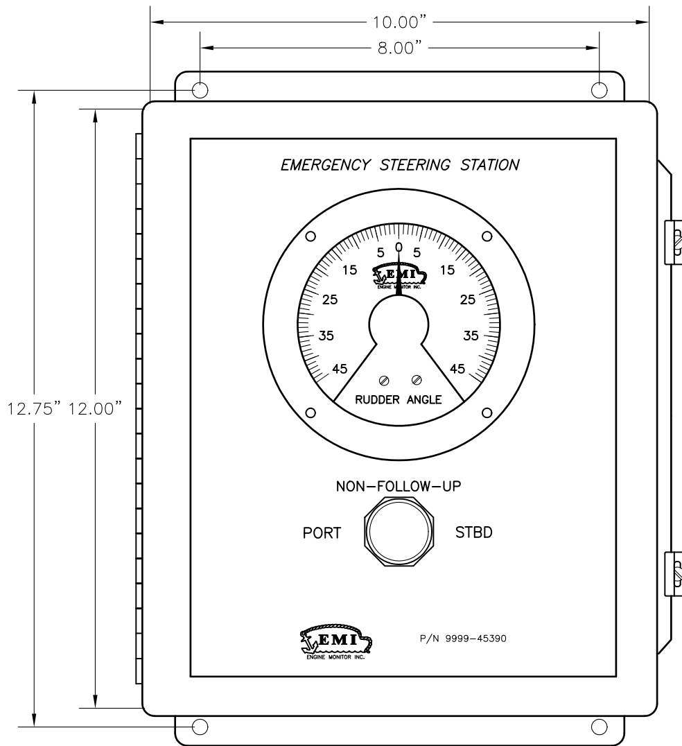
PANEL LAYOUT
