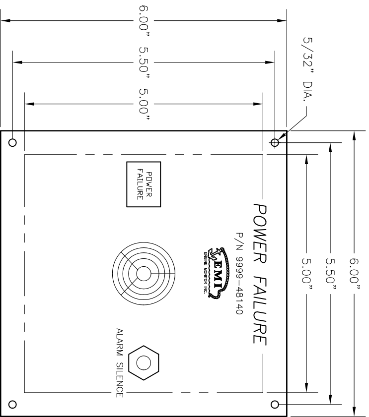
PANEL LAYOUT
